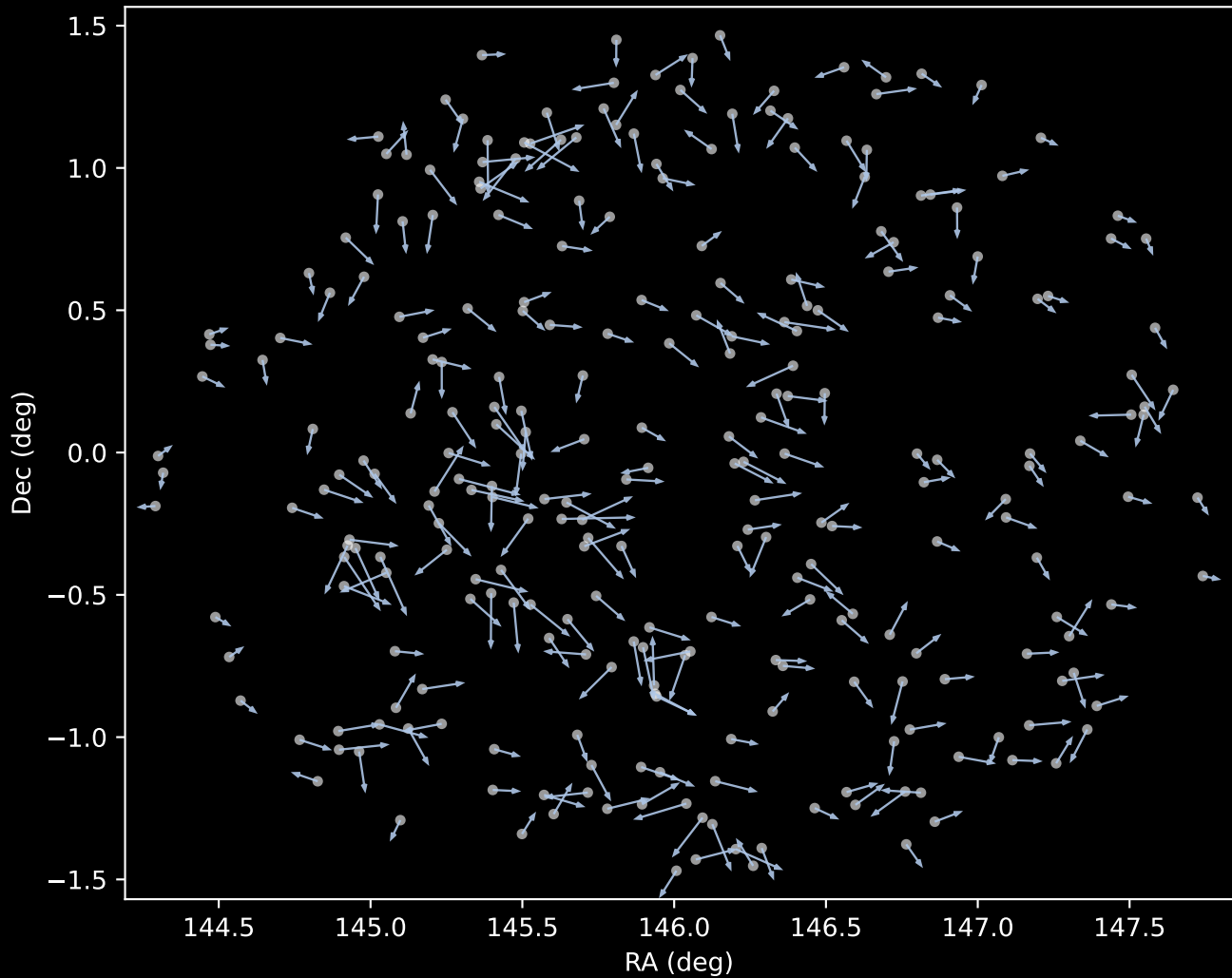
APOGEE DR17 Cluster 1 Proper Motion Vectors (n=267)
