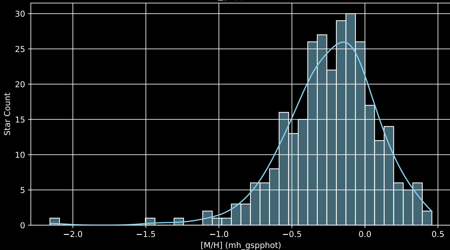
APOGEE DR17 Field: [178-48_MGA [M/H] (mh_gspphot) (n= 299)
