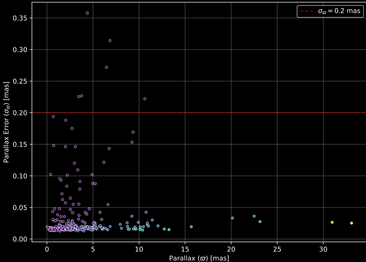
APOGEE DR17 Field: [178-48_MGA] Parallax Quality (n= 303)
