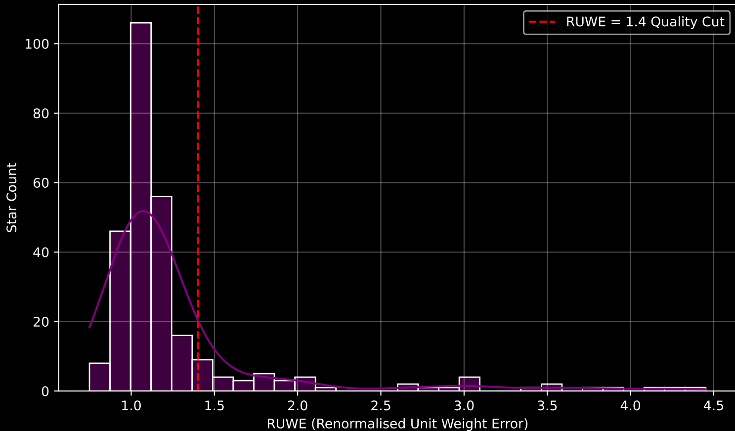
GAPOGEE DR17 Field [178-48_MGA] RUWE Distribution (n= 277)
