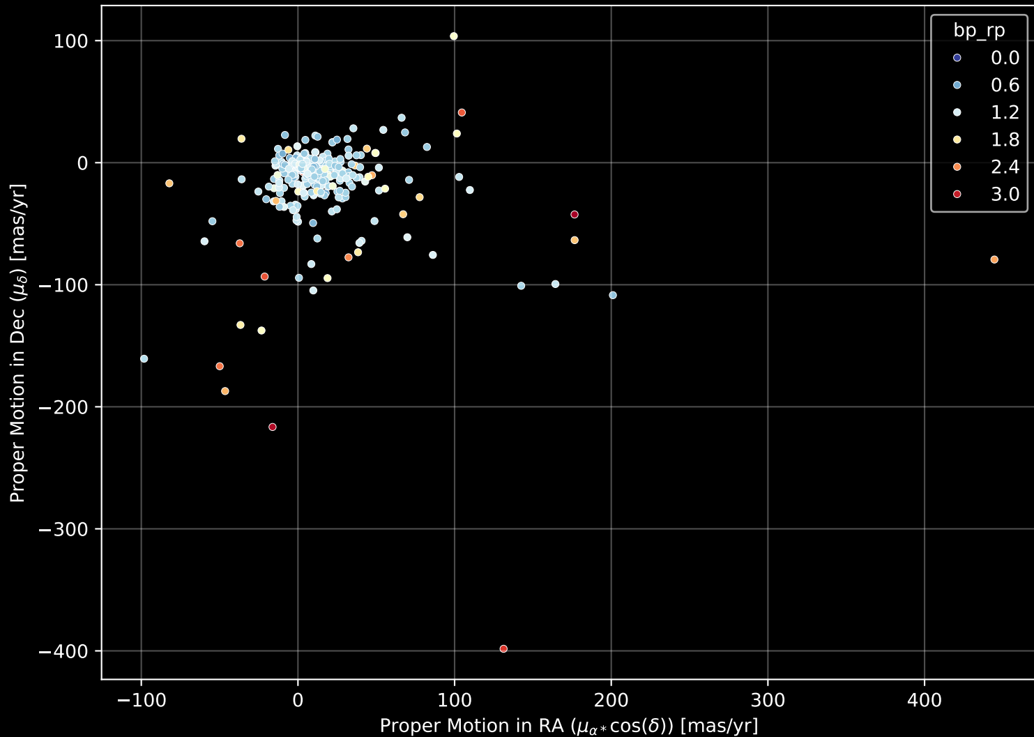
APOGEE DR17 Field: [178-48_MGA] Proper Motion Diagram (n= 303)
